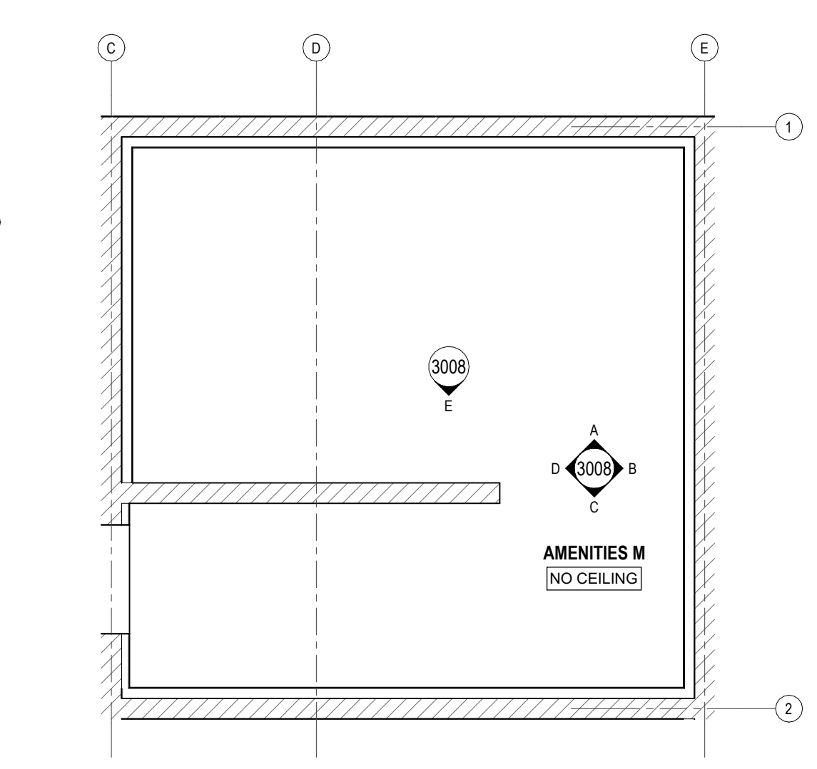
2 REFLECTED CEILING PLAN AMENITIES M Scale: 1:50
