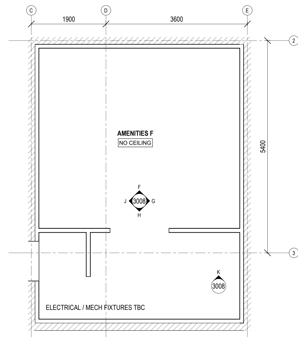
4 REFLECTED CEILING PLAN AMENITIES F Scale: 1:50
